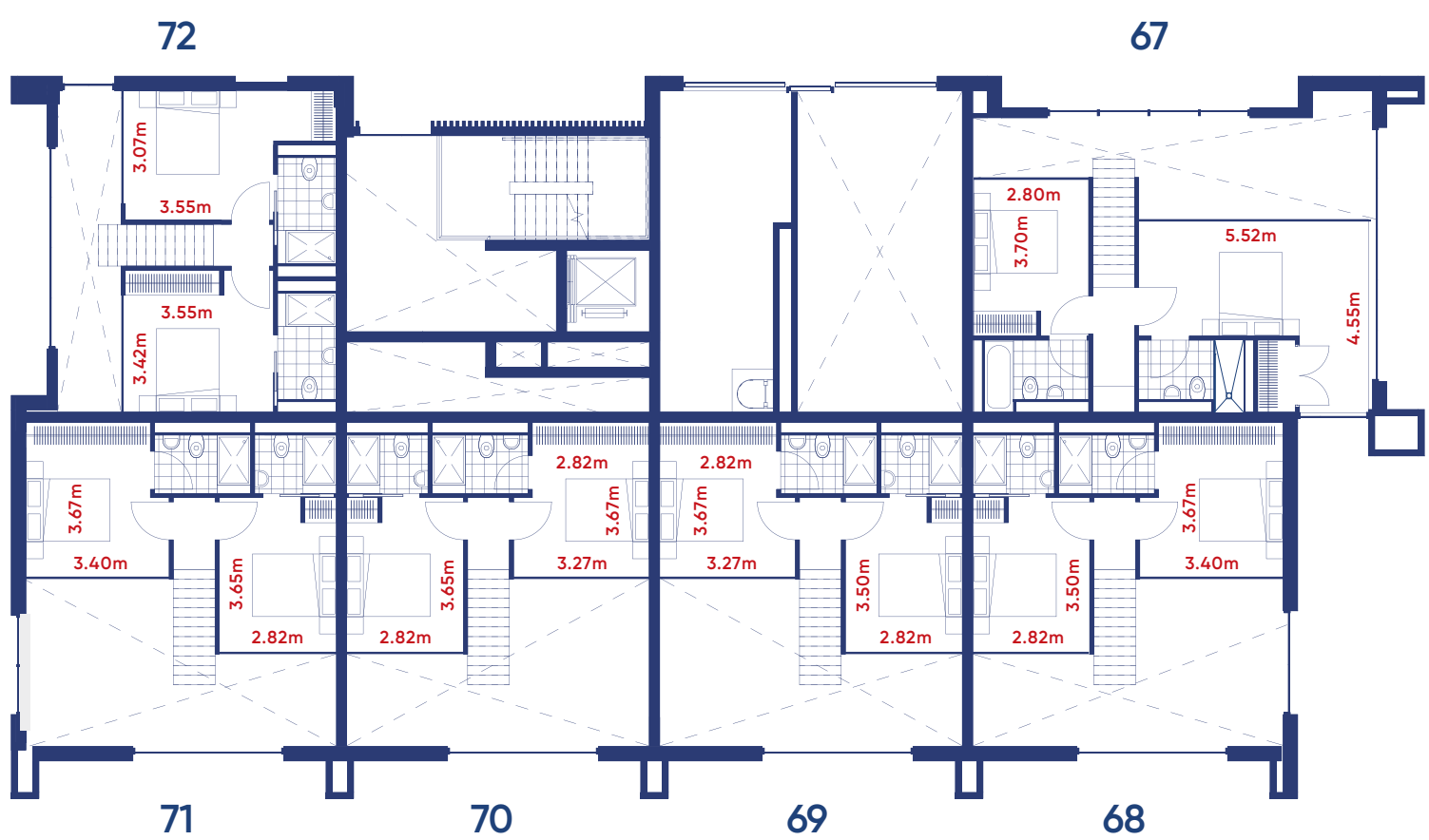
Mezzanine plan
